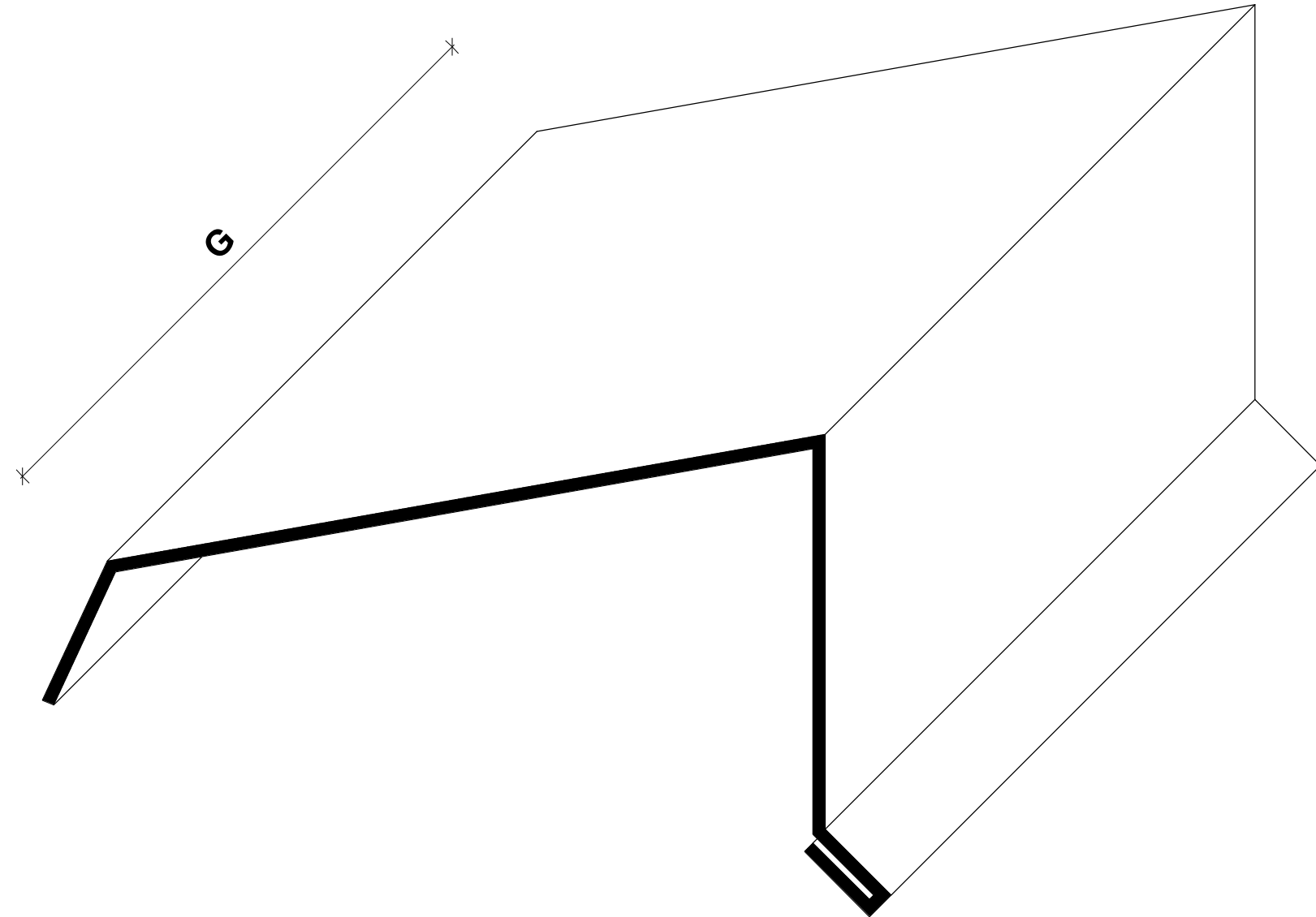
Murkrone 3 3D 1:1
